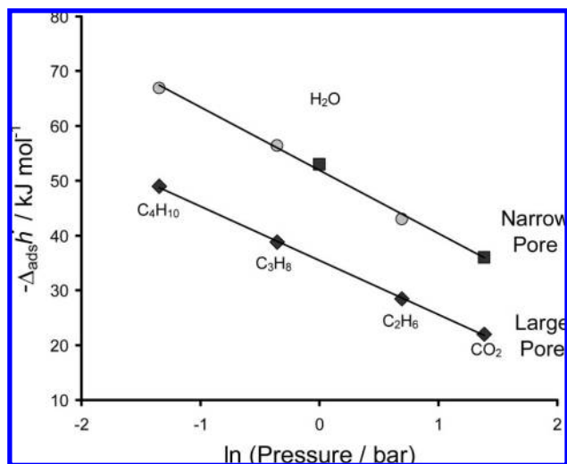
Figure 5. Enthalpies of adsorption as a function of \ln(p) where p corresponds to the pressure range of the 'narrow–large' pore transition for carbon dioxide, water, and the C2–C4 hydrocarbons determined from the isotherms. Diamonds: initial enthalpies measured in the large pore form of MIL53(Cr). Squares: enthalpy measured during the filling of the narrow pore. Circles: simulated enthalpies for narrow pore filling.
